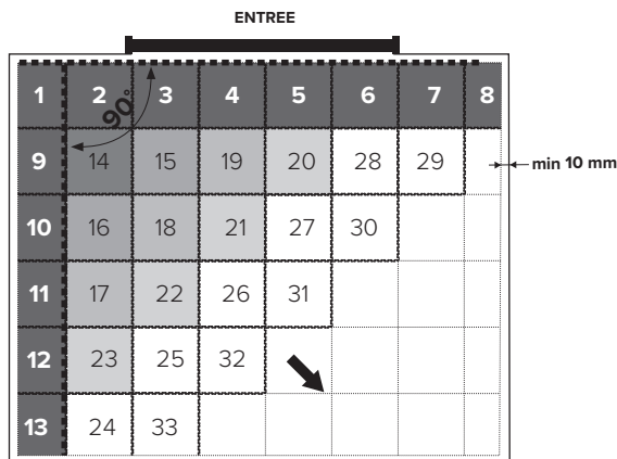
Fig. 2 Pose Fortelock INVISIBLE, INVISIBLE XL, BUSINESS
