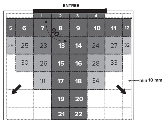
Fig. 1 Pose Fortelock INDUSTRY, INDUSTRY ULTRA, XL
